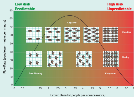
Crowd density versus crowd flow rate
